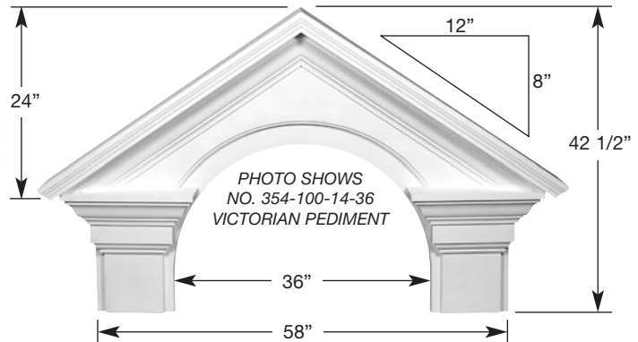
354-100-14-40 Victorian Pediment
