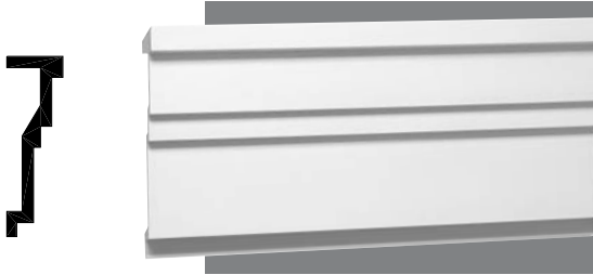
550-476-8 Moulding Ht.: 13 1/8" Length: 8' Proj.: 5"
