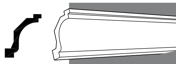
550-370-16 Moulding Ht.: 5 1/2" Length: 16' Proj.: 4 5/8"
