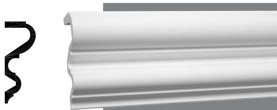
550-312-10 Moulding Ht.: 12 5/16" Length: 10' Proj.: 4 5/8"
