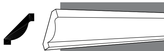
550-450-16 Moulding Ht.: 3 1/8" Length: 16' Proj.: 3"
