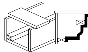
Miter Box cut-a-way & blocking for smaller profiles
