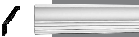
550-204-16 Moulding Ht.: 3 3/8" Length: 16' Proj.: 2 1/8"
