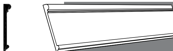
550-470-16 Moulding Ht.: 8 7/8" Length: 16' Proj.: 1 3/8"
