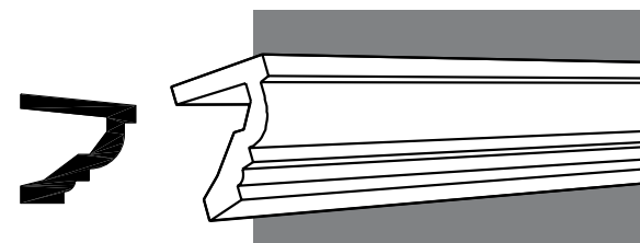
550-480-16 Moulding Ht.: 9 1/2" Length: 16' Proj.: 10"
