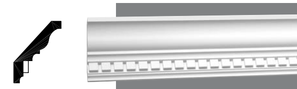
550-466-16 Moulding Ht.: 5 1/4" Length: 16' Proj.: 4"
