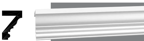
550-142-16 Moulding Ht.: 5 3/8" Length: 16' Proj.: 3 1/2"
