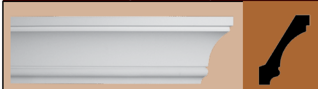
MMLD 1036-16 Hght 6-1/4" x Proj 4-3/8" x 16'
