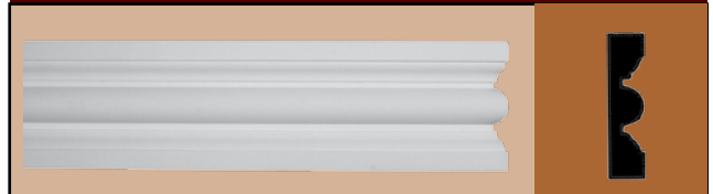
MMLD 1027-16 Hght 4-5/8" x Proj 3-1/2" x 16'
