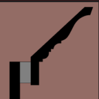
Hght 9-1/4" x Proj 7-5/8" x 16'
