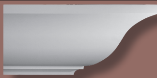
MMLD 2134-12 Hght 17-3/4" x Proj 13-5/8" x 12'
